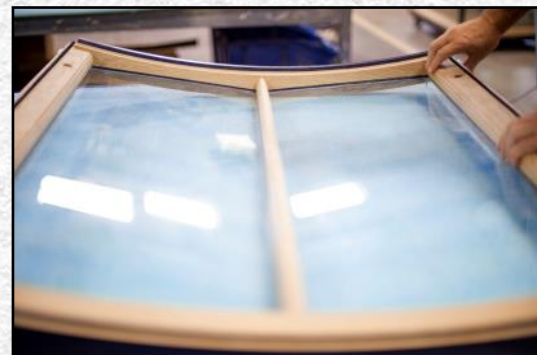
Detail of sash featuring angled TDL bar configuration with flat glass.
